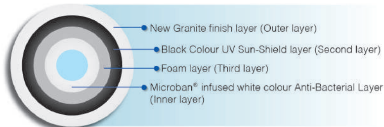
Cross-section of 'Ganga Granito 4 Layer' Water Tank
