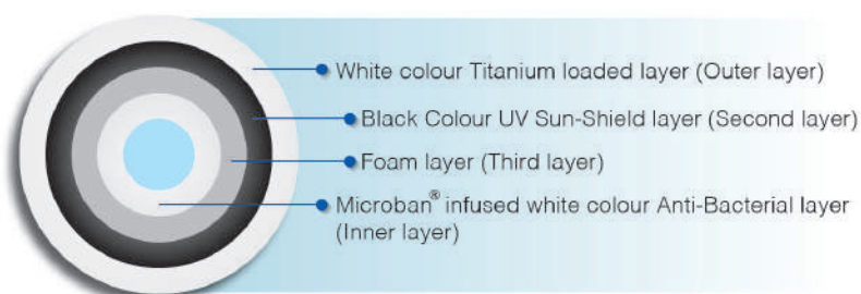
Cross-section of 'Ganga Cool 4 Layer' Water Tank
