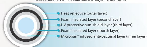
Cross-section of 'Vectus Euro 5 Layer' water tank
