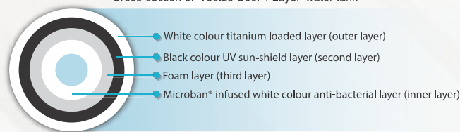
Cross-section of 'Vectus Cool 4 Layer' water tank
