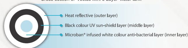
Cross-section of 'Vectus Mini 3 Layer' water tank
