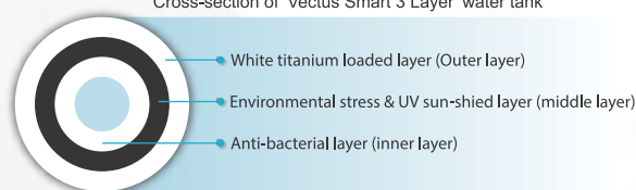
Cross-section of 'Vectus Smart 3 Layer' water tank
