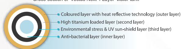
Cross-section of 'Vectus Next 4 Layer' water tank
