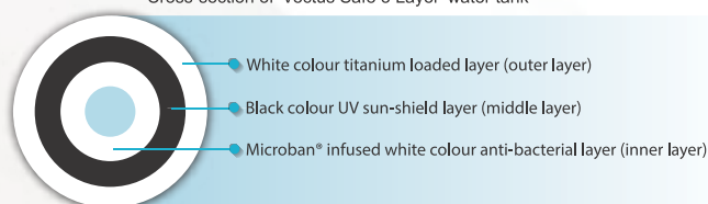
Cross-section of 'Vectus Safe 3 Layer' water tank
