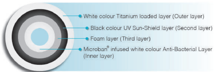
Cross-section of 'Vectus Cool 4 Layer' Water Tank
