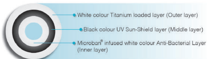
Cross-section of 'Vectus Safe 3 Layer' Water Tank
