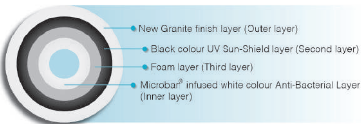
Cross-section of 'Vectus Granito 4 Layer' Water Tank
