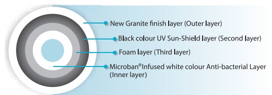
Cross-section of 'Waterwell Granito 4 Layer' Water Tank
