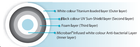
Cross-section of 'Waterwell Italian 4 Layer' Water Tank
