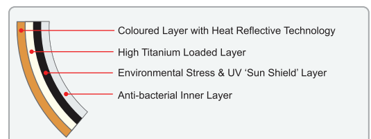
Cross-section of 'Waterwell Wonder 4 Layer' Water Tank
