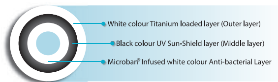
Cross-section of 'Waterwell Health 3 Layer' Water Tank
