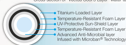
Cross-section of "Vectus Cool 5 Layer" water tank
